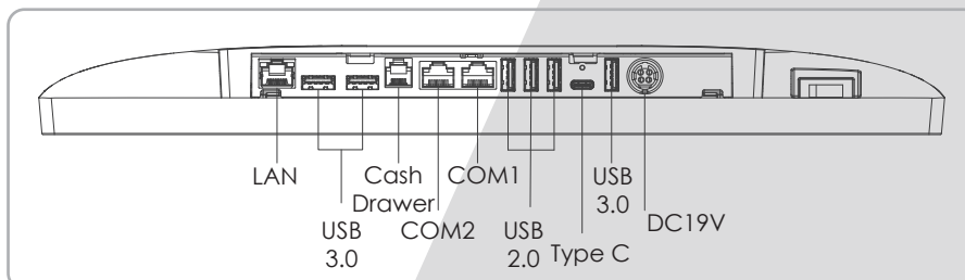
IO Panels (PE24/PE26)
